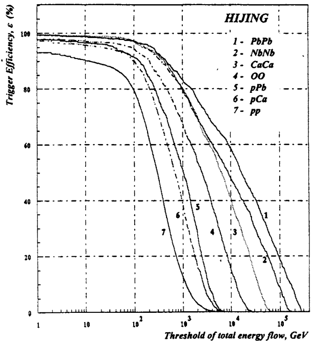
Fig.3. The efficiency of the event selection vs the total energy threshold for nucleus-nucleus (PbPb, NbNb, CaCa, OO), proton-nucleus ( p Pb, p Ca), and proton-proton collisions at 5 TeV/nucleon in the centre of mass system
