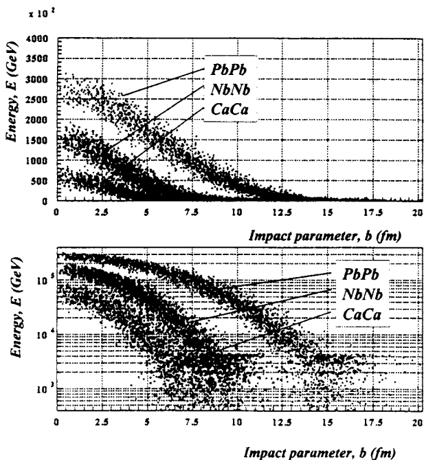
Fig.1. Dependence of the energy flow per event in the very forward calorimeter, E (GeV) vs the nuclear collision impact parameter, b (fm) in the HIJING model
