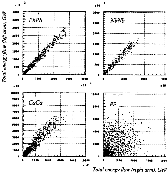
Fig.2. The correlation between the detected energy in two pseudorapidity regions -5 < \eta < -3 and 3 < \eta < 5 for PbPb interaction at 5 TeV/nucleon in the centre of mass system
