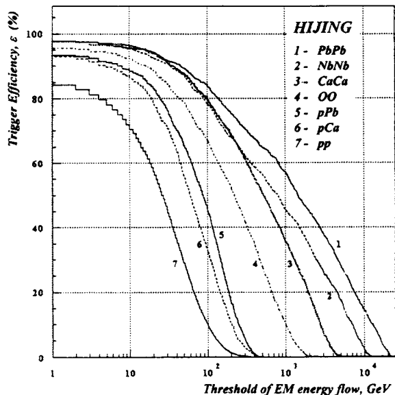
Fig.4. The efficiency of the event selection vs the electromagnetic energy threshold for nucleus-nucleus (PbPb, NbNb, CaCa, OO), proton-nucleus ( p Pb, p Ca), and proton-proton collisions at 5 TeV/nucleon in the centre of mass system
